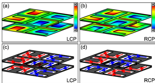
Fig. 4. (Color online) False-color plots of the axial component of the local magnetic field in two planes cutting through the SRR layers for (a) LCP incidence at 3.2\ \mu\text{m} wavelength and (b) for RCP incidence at 2.5\ \mu\text{m} . Schemes of the corresponding underlying electric currents within the SRR are shown in (c) and (d), respectively.
