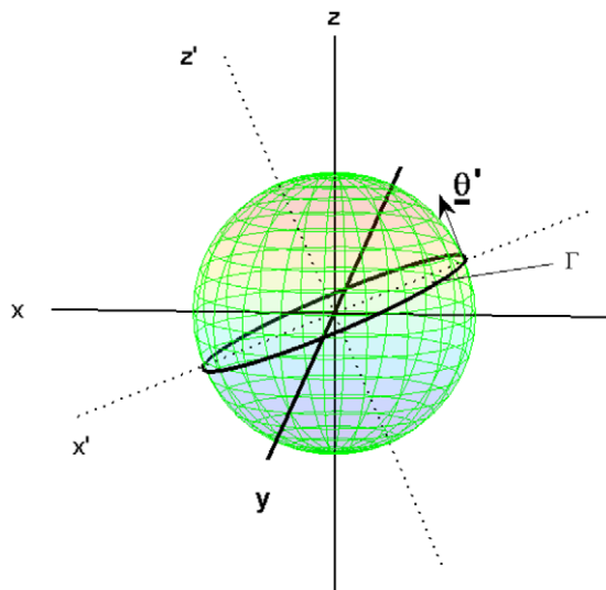
Fig. 2. A sphere rotated about the y -axis by an angle \beta . The x -axis is mapped to the x' -axis and the z -axis is mapped to z' -axis. \Gamma is the equator on the rotated sphere and \underline{\theta}' is the unit vector in the \theta' direction in the rotated frame.
