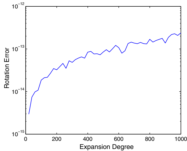
Fig. 3. A plot of error in rotation as a function of expansion degree using the projection-based scheme.
