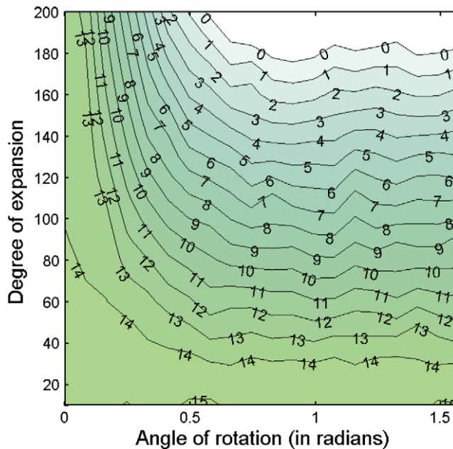
Fig. 1. A plot of accuracy as a function of expansion degree (y-axis) and rotation angle (x-axis). Shown are the contours of -\log_{10}(E) with E defined in (12) – that is, the number of digits of accuracy.
