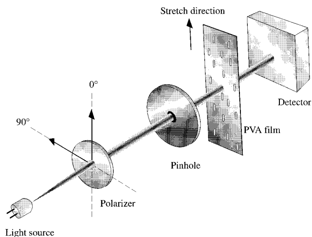
Figure 1. Optical set up. At a polarization angle \Psi = 0^\circ the electric field of the light is polarized parallel to the stretch direction, whereas at a polarization angle \Psi = 90^\circ the electric field of the light is polarized perpendicular to the stretch direction.
