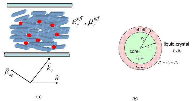
Fig. 1. (Color online) Homogeneous or planar aligned nematic liquid crystal containing a core-shell (coated) nanospheres sample. An applied ac electric field or a magnetic field can switch the director axis of the liquid crystal from parallel to perpendicular to the cell windows. (b) Cross section of the core [ \mu_1, \epsilon_1 ]-shell [ \mu_2, \epsilon_2 ] nanosphere with the liquid crystal host [ \mu_3, \epsilon_3 ].
