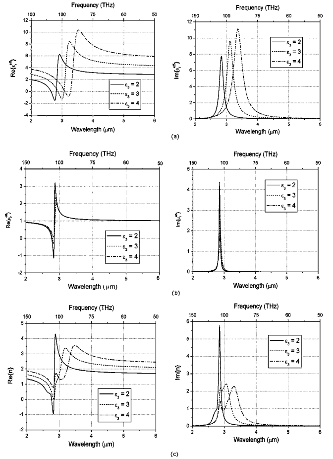
Fig. 2. Calculated real and imaginary part of the complex effective (a) permittivity, (b) permeability, and (c) refractive index of the NDLC as a function of liquid crystal host permittivity in the optical frequency interval between 50 and 150 THz (wavelength between 6 and 2 \mu\text{m} ).
